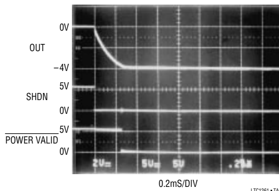
Waveforms for -4\text{V} Generator with Power Valid
