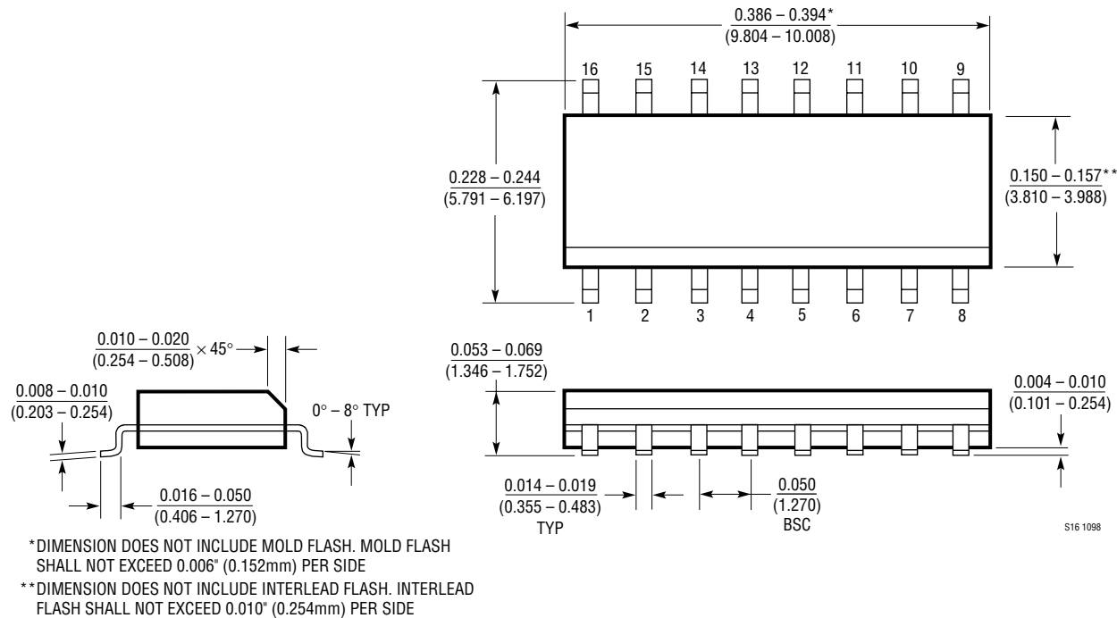
S Package 16-Lead Plastic Small Outline (Narrow 0.150) (LTC DWG # 05-08-1610)
