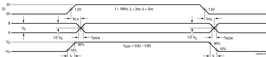
Figure 4. Driver Propagation Delays
