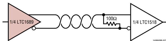
Figure 9. Point-to-Point Transmission
