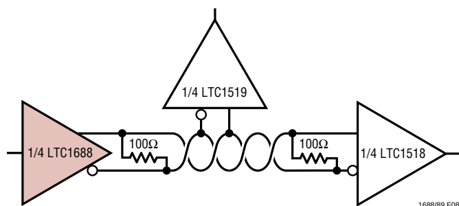
Figure 8. Multipoint Transmission
