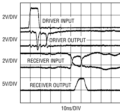
Figure 11. 8ns Pulse Over 25 Feet Category 5 UTP
