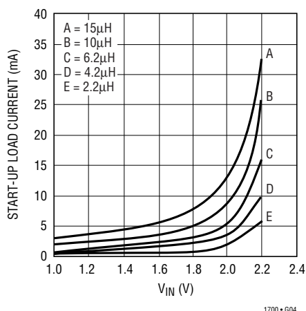
Figure 4. Start-Up Load Current
