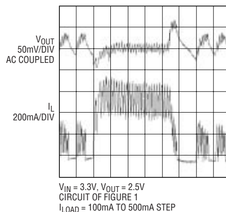
Transient Response
