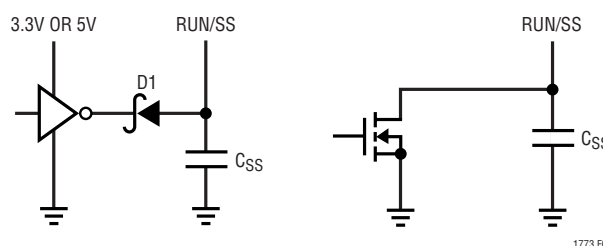
Figure 4. RUN/SS Pin Interfacing
