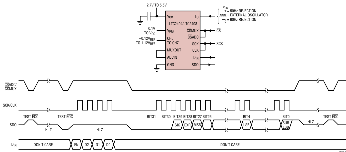
Figure 7. External Serial Clock Timing Diagram
