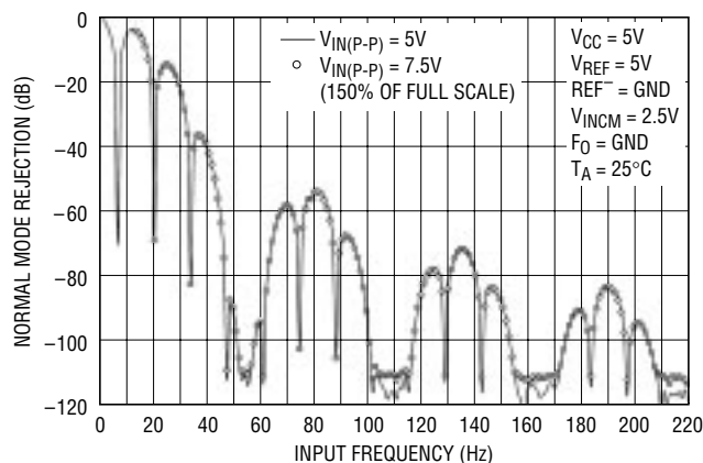
Figure 39. Measured Input Normal Mode Rejection vs Input Frequency (LTC2411-1)
