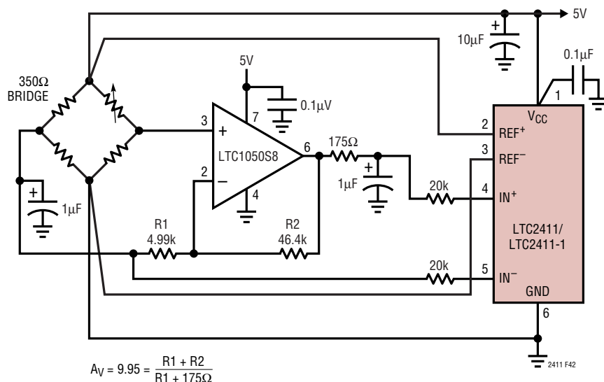
Figure 42. Bridge Amplification Using a Single Amplifier
