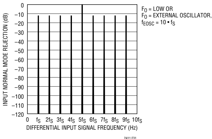
Figure 31. Input Normal Mode Rejection, Internal Oscillator and F 0 = LOW or External Oscillator
