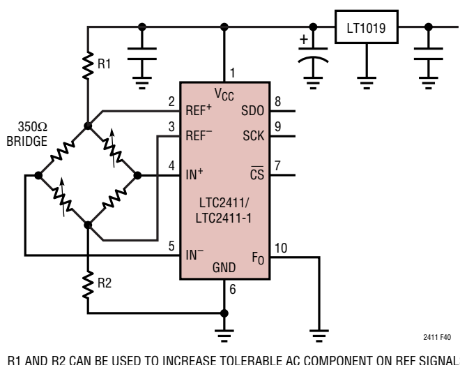
Figure 40. Simple Bridge Connection
