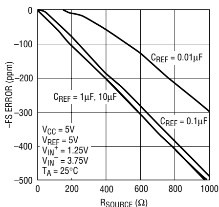
Figure 14. -FS Error vs R_{\text{SOURCE}} at \text{REF}^+ or \text{REF}^- (Large C_{\text{REF}} )
