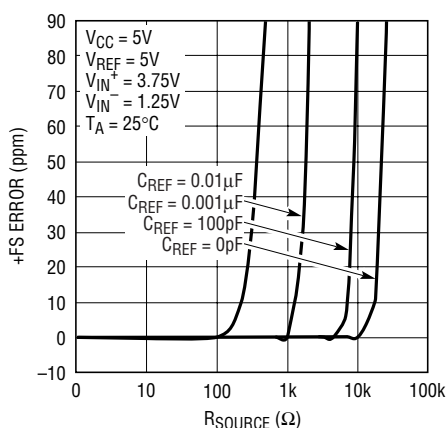
Figure 11. +FS Error vs R_{\text{SOURCE}} at \text{REF}^+ or \text{REF}^- (Small C_{\text{REF}} )
