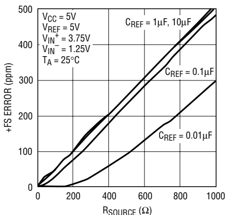
Figure 13. +FS Error vs R_{\text{SOURCE}} at \text{REF}^+ or \text{REF}^- (Large C_{\text{REF}} )
