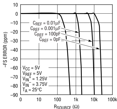
Figure 12. -FS Error vs R_{\text{SOURCE}} at \text{REF}^+ or \text{REF}^- (Small C_{\text{REF}} )
