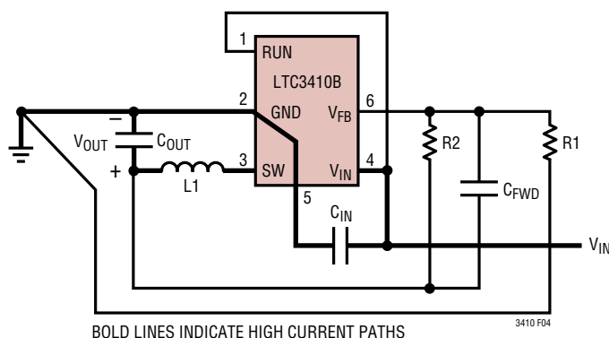
Figure 4. LTC3410B Layout Diagram
