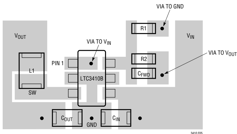
Figure 5. LTC3410B Suggested Layout
