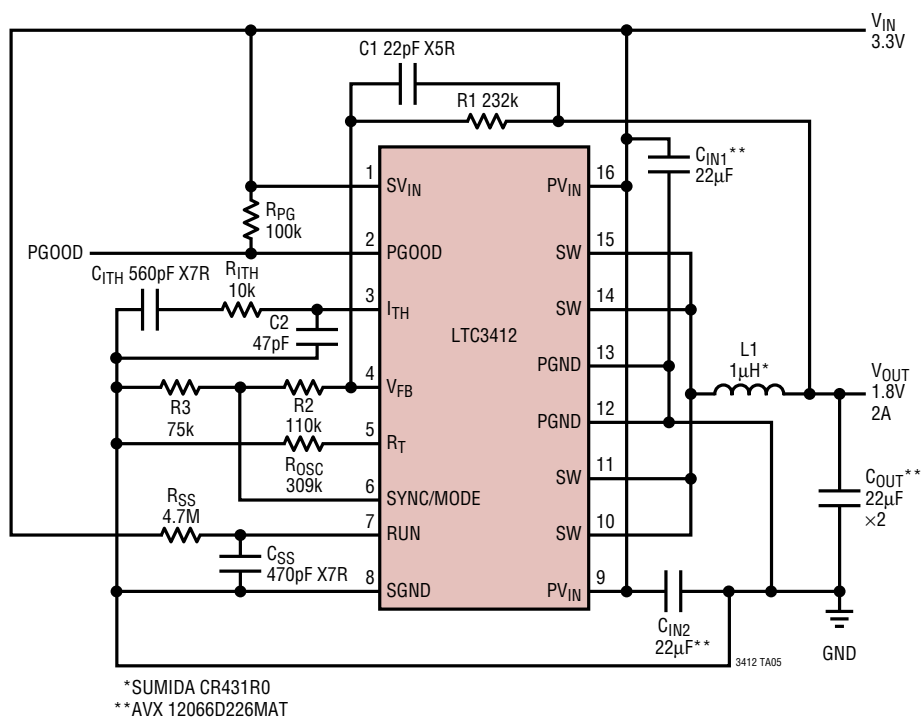
1.8V, 2.5A Step-Down Regulator at 1MHz, Burst Mode Operation
