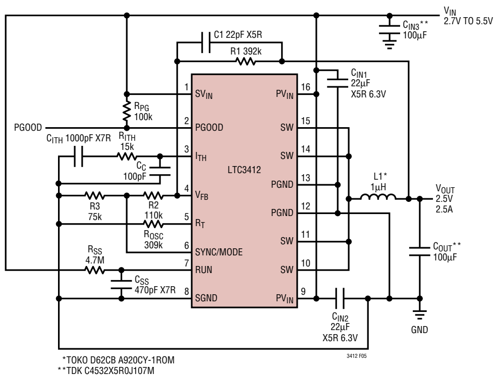
2.5V, 2.5A Regulator Using All Ceramic Capacitors
