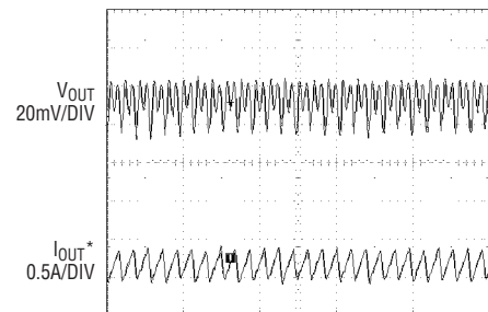
Constant Frequency (Burst Inhibit) Operation (Figure 13)
