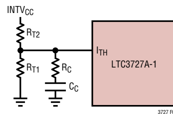
Figure 8. Active Voltage Positioning Applied to the LTC3727A-1
