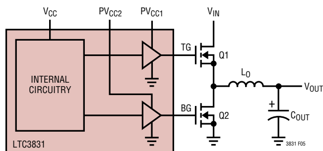
Figure 5. Supplies Input
