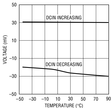
Shutdown Threshold (DCIN – V CC )
