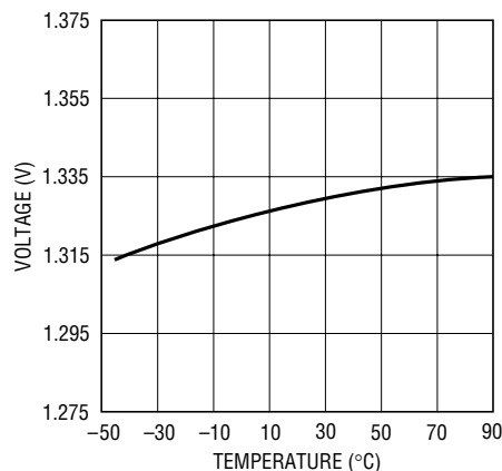
Automatic Recharge Threshold (per Cell)
