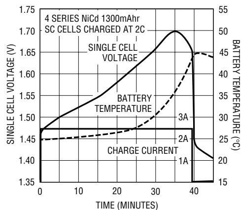
NiCd Charge at 2C
