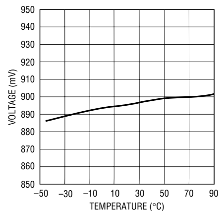
Minimum Fast Charge Threshold (per Cell)
