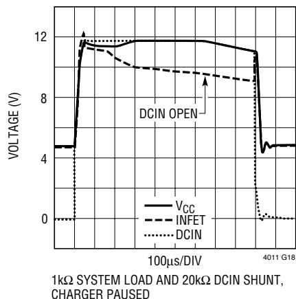
PowerPath Switching
