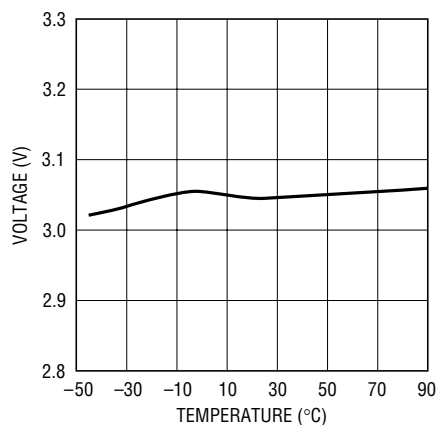
Thermistor Disable Threshold
