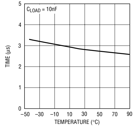
INFET OFF Delay
