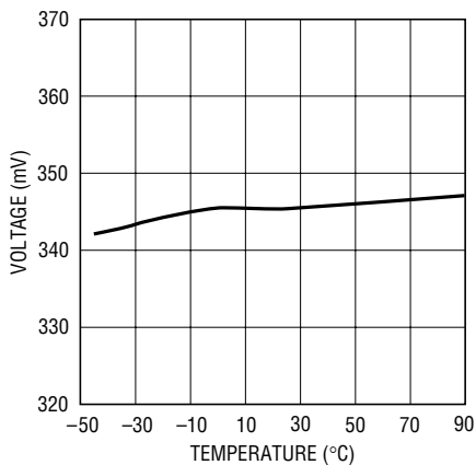
Battery Present Threshold (per Cell)
