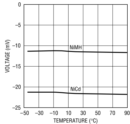
-ΔV Termination (per Cell)
