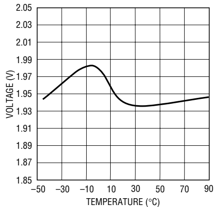
Battery Overvoltage Threshold (per Cell)
