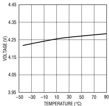
Undervoltage Lockout Threshold
