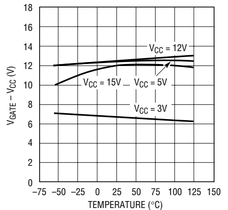
V_{\text{GATE}} - V_{\text{CC}} vs Temperature
