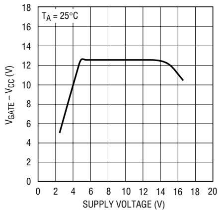
V_{\text{GATE}} - V_{\text{CC}} vs Supply Voltage
