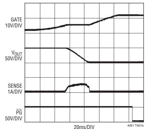
Start-Up Behavior
