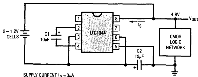
Generating CMOS Logic Supply from 2 Mercury Batteries
