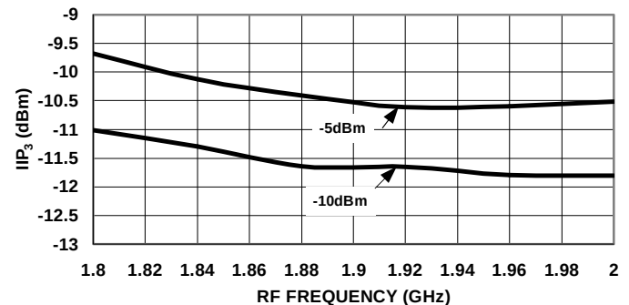
Input IP 3 vs. Frequency LO = -10dBm, -5dBm, V_{DD} = 3.0V
