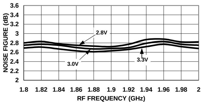
Noise Figure vs. Frequency V_{DD} = 2.8V, 3.0V, 3.3V, LO = -10dBm
