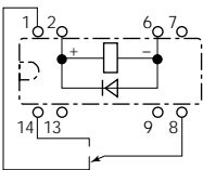
SPDT-1 Form C w/diode
