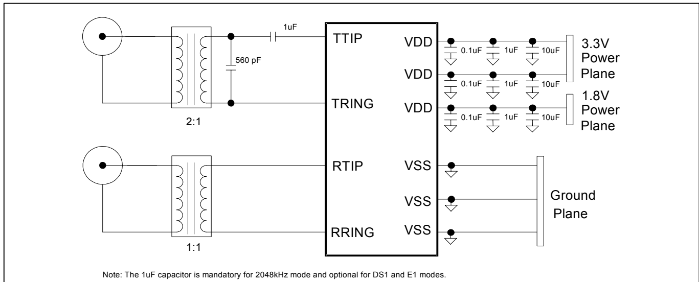
Figure 7-10. BITS Transceiver External Components
