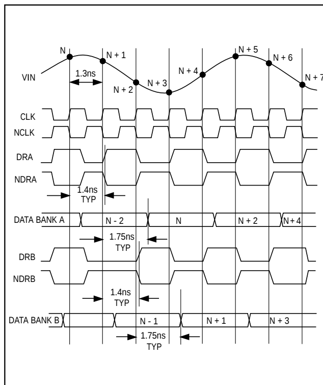
Figure 2. Timing Diagram
