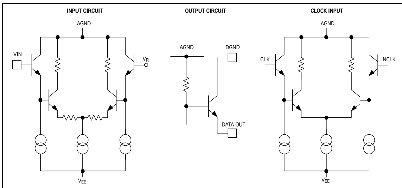
Figure 3. Subcircuit Schematics
