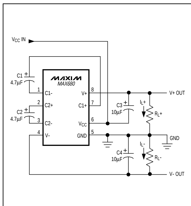
Figure 1. Test Circuit
