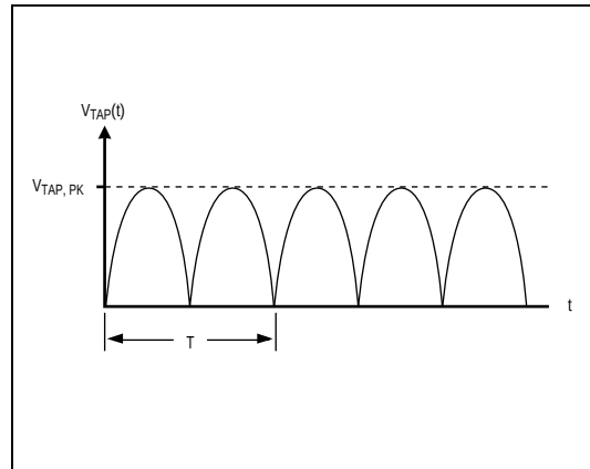
Figure 5. Voltage at the Center Tap of T1
