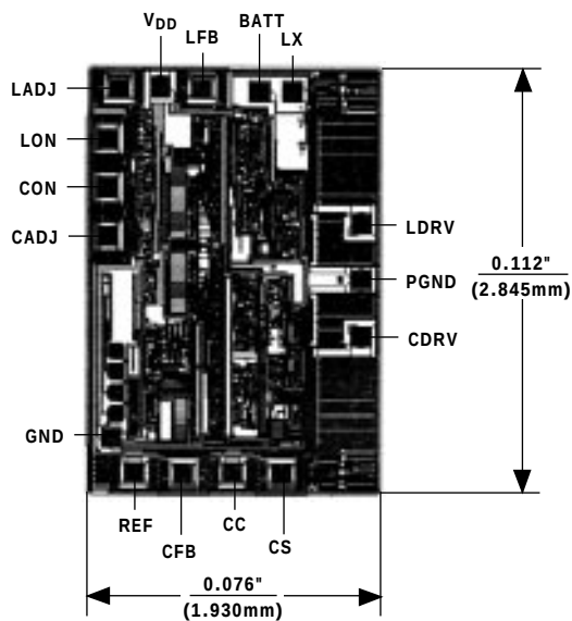
Chip Topography
