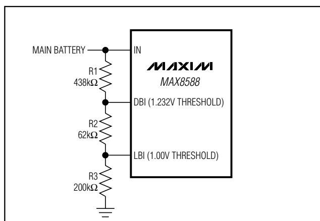
Figure 3. Setting the Low-Battery and Dead-Battery Thresholds with One Resistor Chain. The values shown set a DBI threshold of 3.3V and an LBI threshold of 3.5V (no resistors are needed for the factory preset thresholds).
