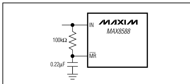
Figure 2. An RC delay connected from IN to \overline{MR} ensures that the 65ms \overline{RSO} release delay remains in effect for any sequence of IN and V7.
