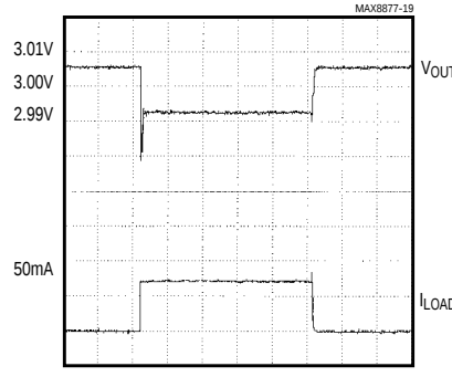
LOAD-TRANSIENT RESPONSE
