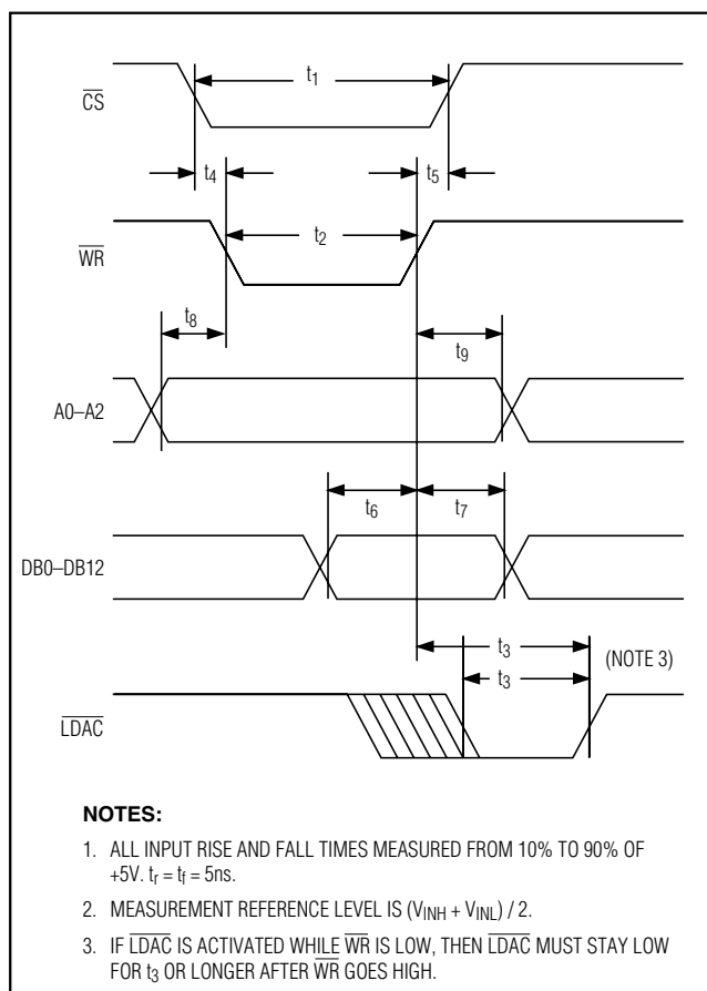
Figure 2a. Digital Timing Diagram
