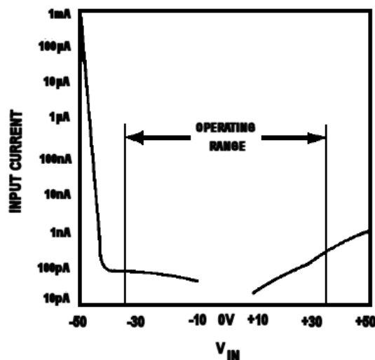
FIGURE 1. INPUT LEAKAGE VS. INPUT VOLTAGE WITH V^+ = V^- = 0V
