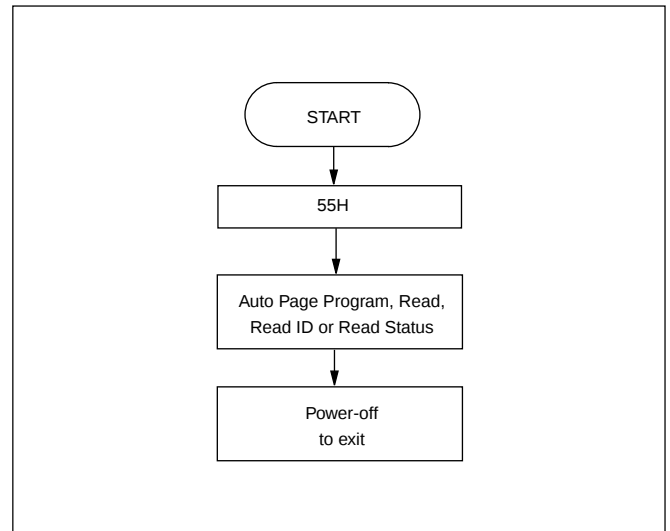
Parallel Mode for Read/Program Flow Chart
