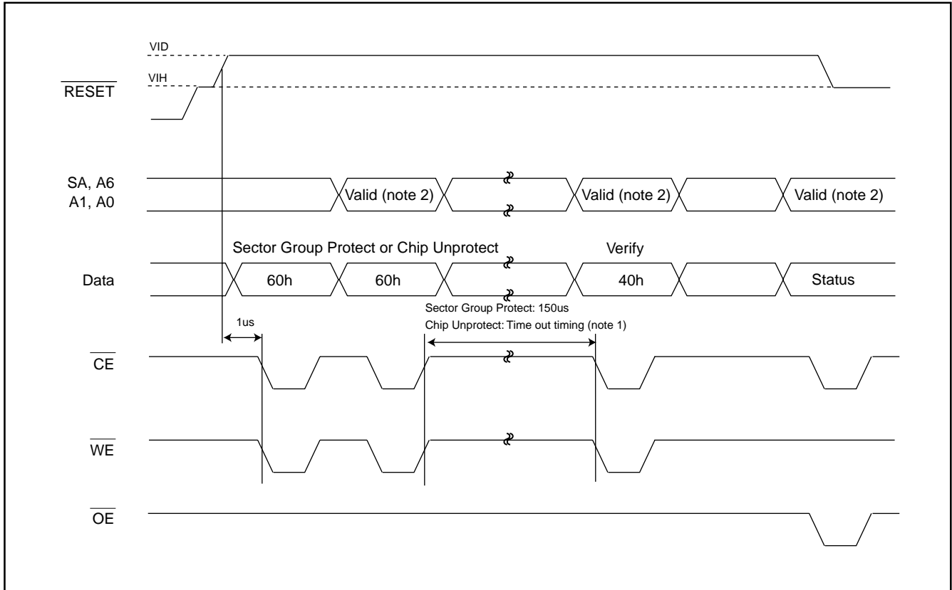
Fig 13. SECTOR GROUP PROTECT/CHIP UNPROTECTED WAVEFORM (RESET Control)
