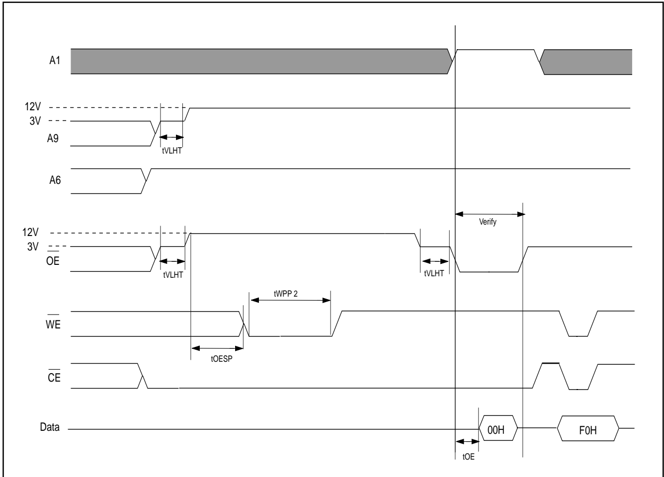
Fig 16. CHIP UNPROTECTED TIMING WAVEFORM(A9, OE Control)
