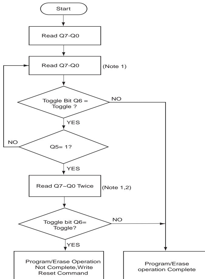
Figure 18. TOGGLE BIT ALGORITHM
