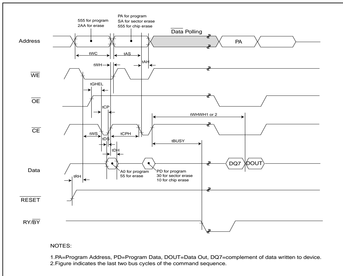
Figure 7. \overline{CE} CONTROLLED PROGRAM TIMING WAVEFORM
