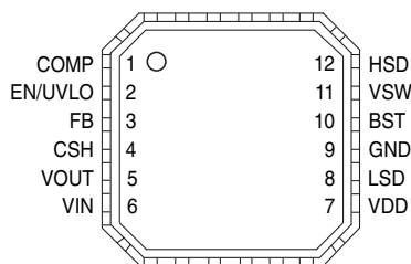
4×4 MLF-12L (ML)
