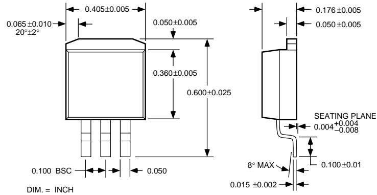
3-Lead TO-263 (U)
