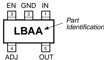
MIC5205BM5 Adjustable Voltage
