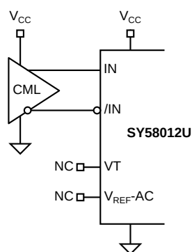
Figure 3d. DC-Coupled CML Input Interface
