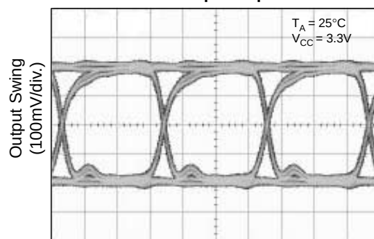
3.2Gbps Output
