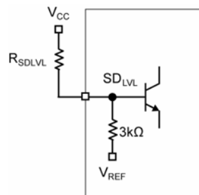
Figure 6. SD_{LVL} Setting Circuit
