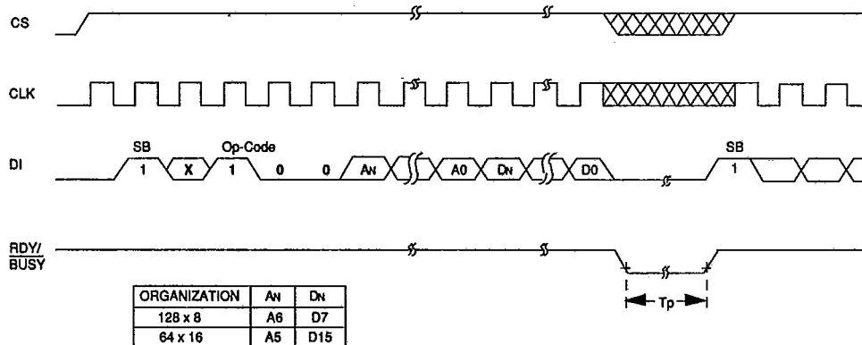
FIGURE 3 - PROGRAM MODE
