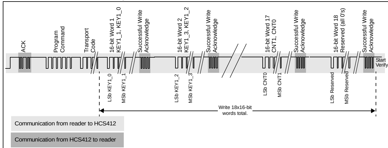
FIGURE 4-10: PROGRAMMING - VERIFICATION
