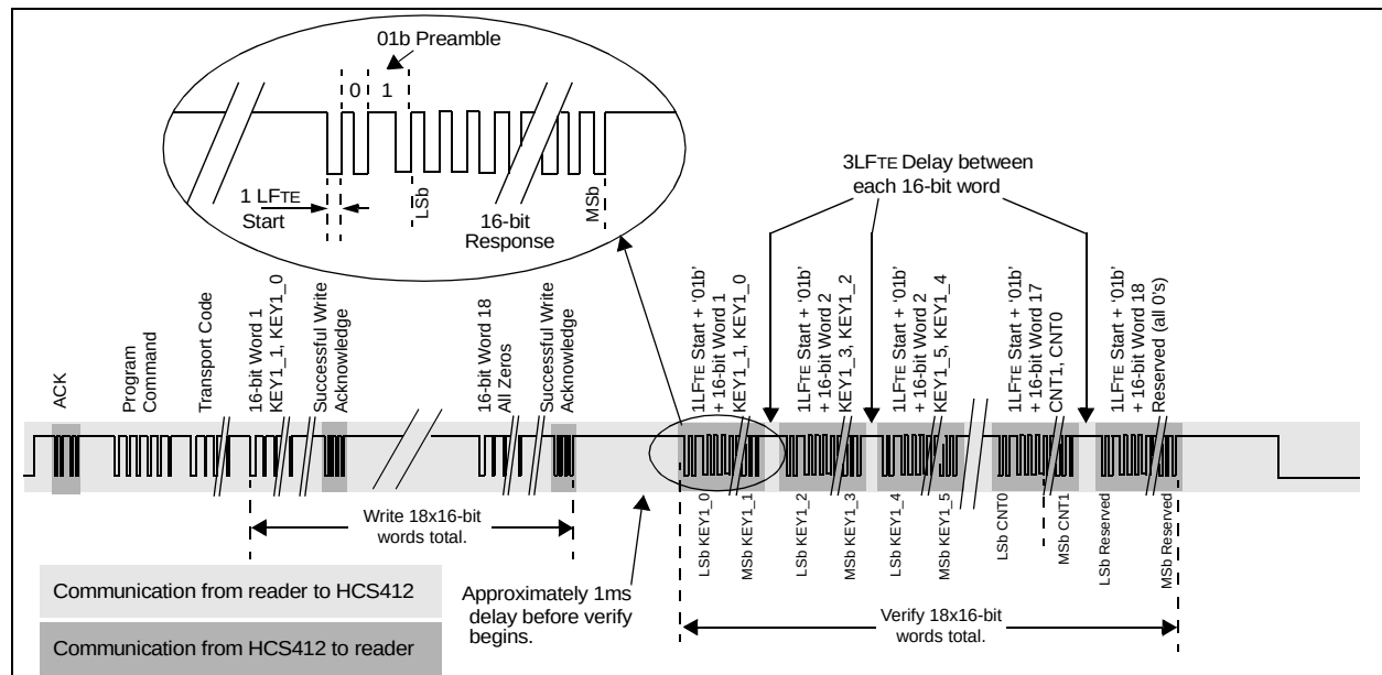
FIGURE 4-10: PROGRAMMING - VERIFICATION
