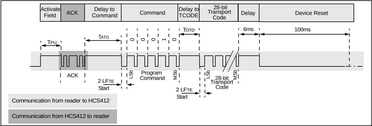
FIGURE 4-7: BULK ERASE
