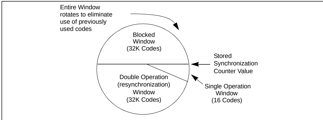
FIGURE 6-3: SYNCHRONIZATION WINDOW
