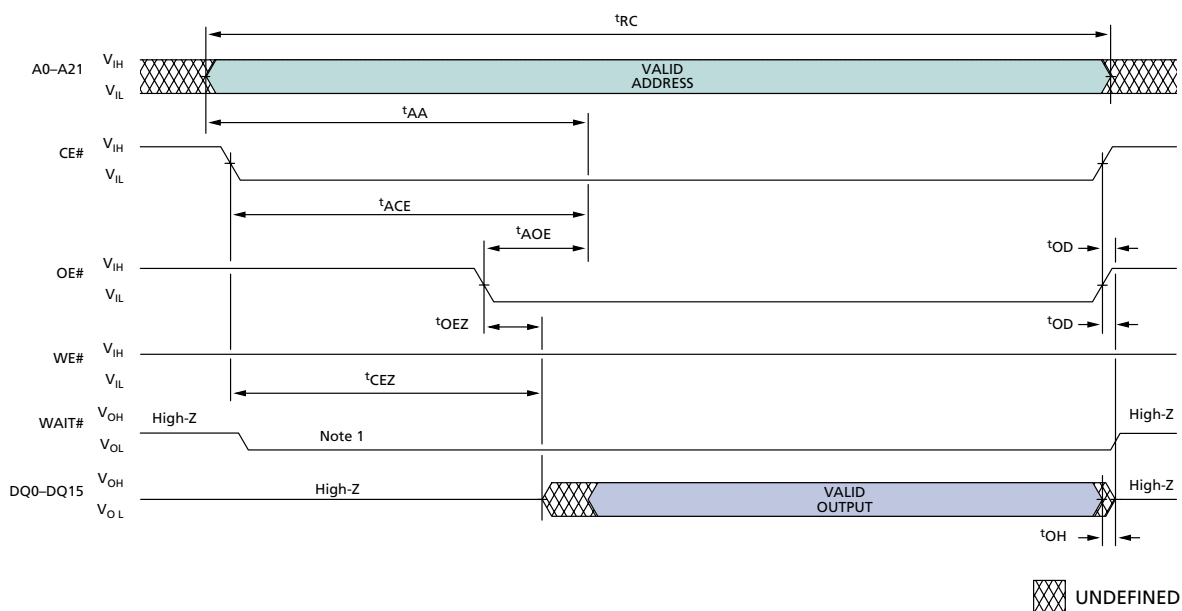
Figure 28: WAIT# Signal in Asynchronous READ Operation
