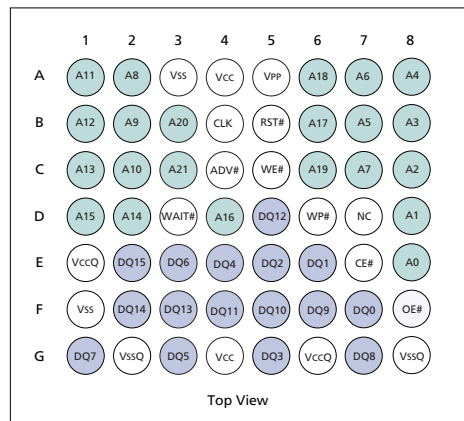
Figure 1: 56-Ball VFBGA
