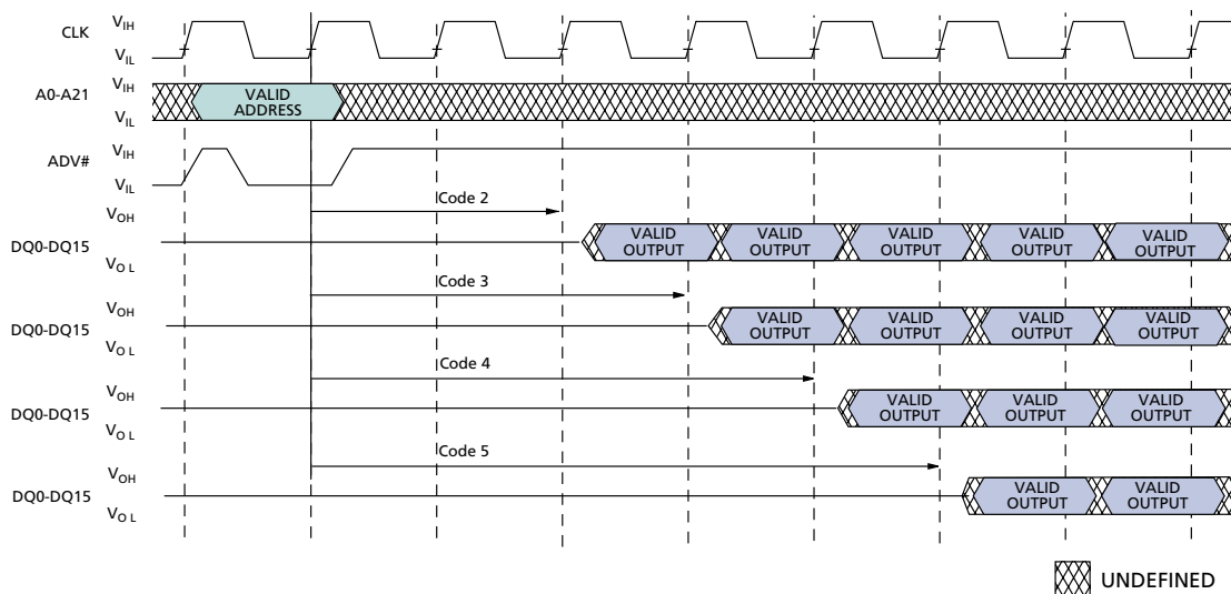
Figure 6: Latency Counter 1
