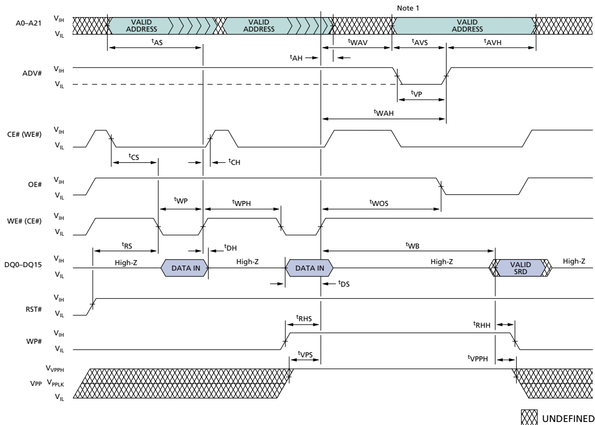
Figure 29: Two-Cycle WRITE Operation
