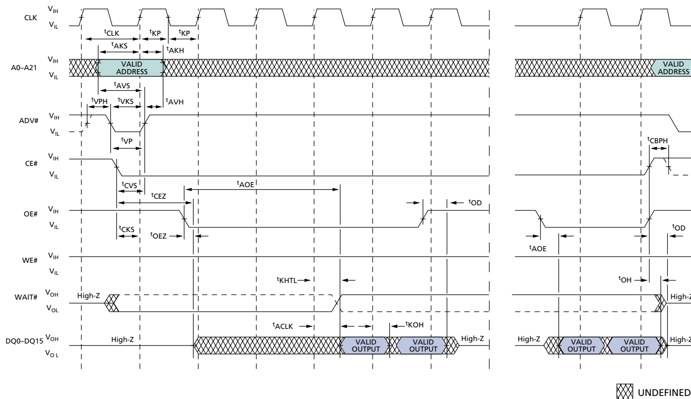
Figure 30: Clock Suspend
