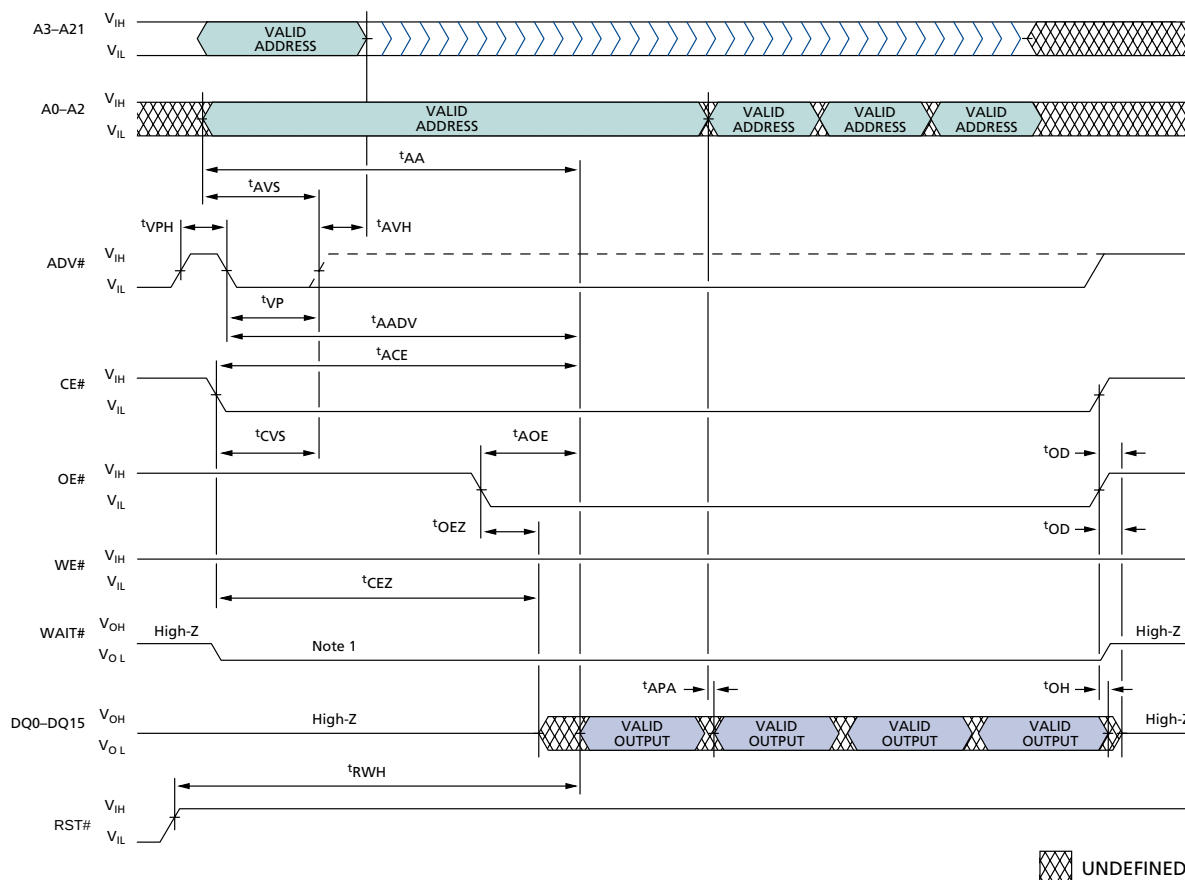
Figure 23: Page Mode READ Operation
