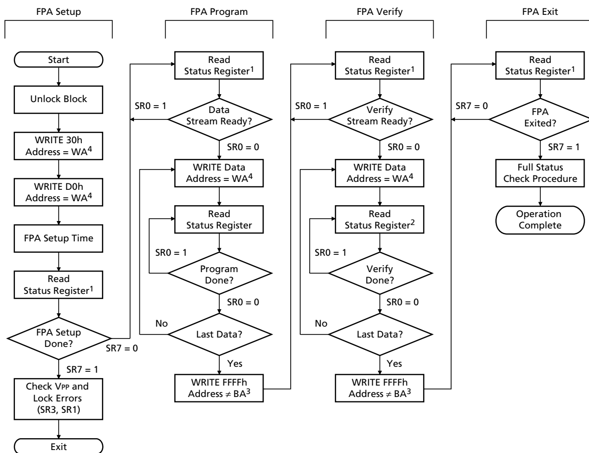
Figure 9: Fast Programming Algorithm (FPA) Flowchart (in-factory only)
