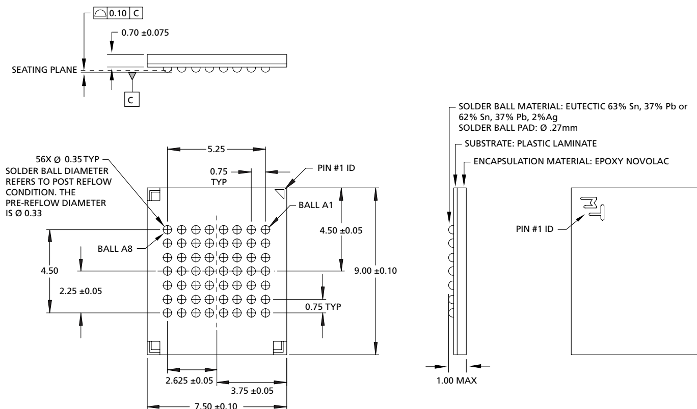
Figure 35: 56-Ball VFBGA
