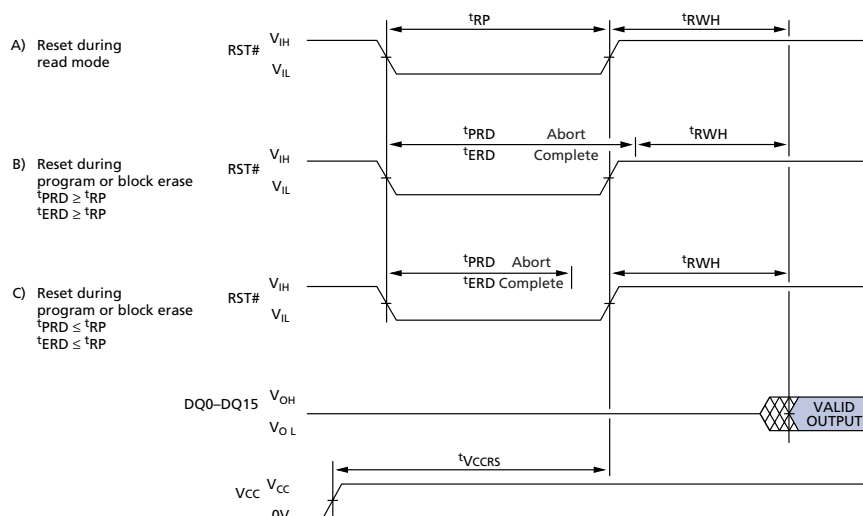
Figure 18: Reset Operations
