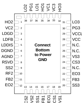
LQ PACKAGE (Top View)
