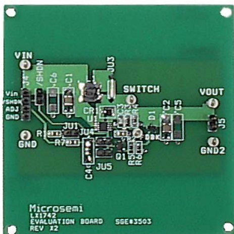
Figure 5 – LXE1742 - LX1742 Circuit Evaluation Board
