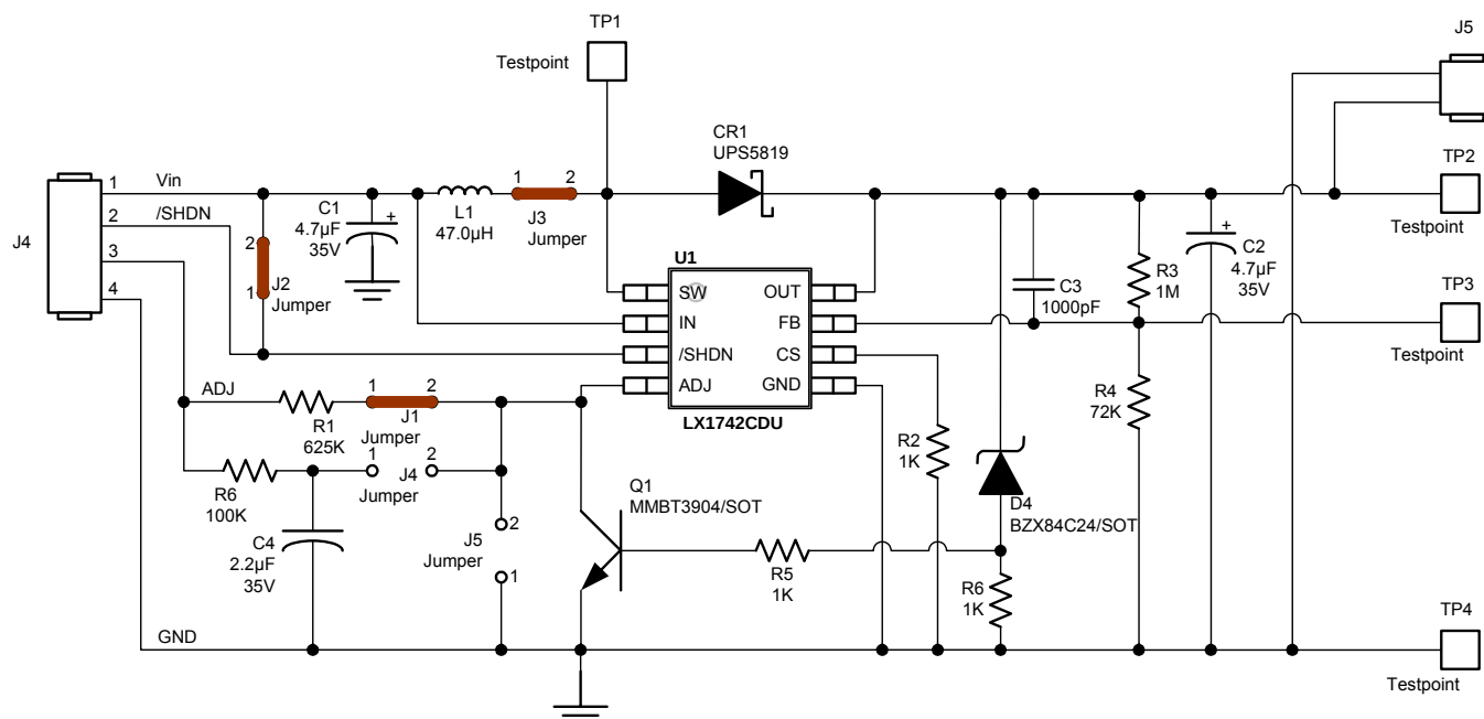
Figure 4 – LXE1742 Boost Evaluation Board Schematic
