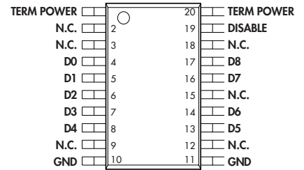
PW PACKAGE (Top View)
