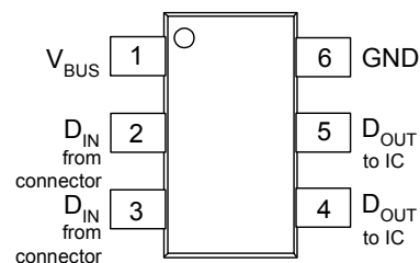
SF PACKAGE (Top View)
