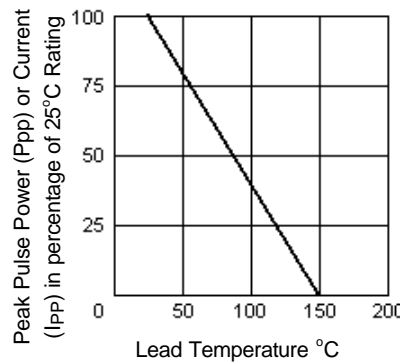
FIGURE 3 Derating Curve
