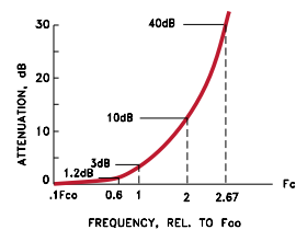
TYPICAL FREQUENCY RESPONSE
