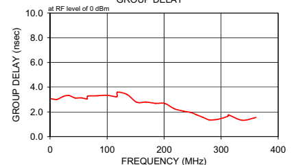
GROUP DELAY
