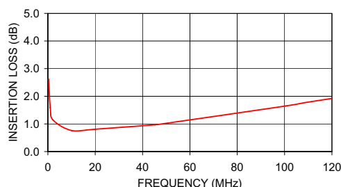
TMO13-1T INSERTION LOSS
