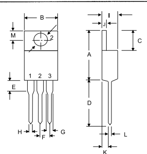
TO-220AB
