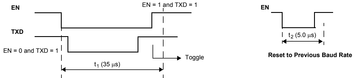
Figure 11. Fast Baud Rate Selection (Toggle Function)
