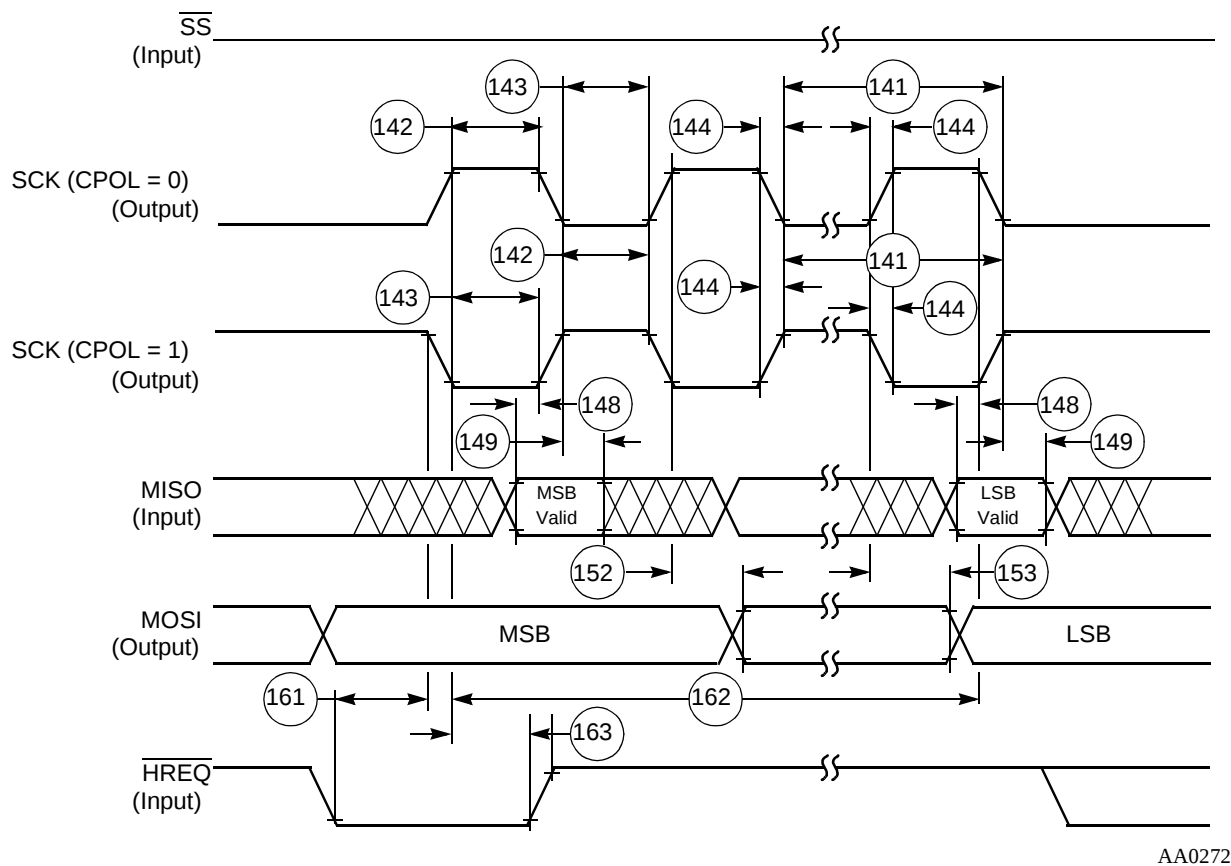
Figure 2-19. SPI Master Timing (CPHA = 1)
