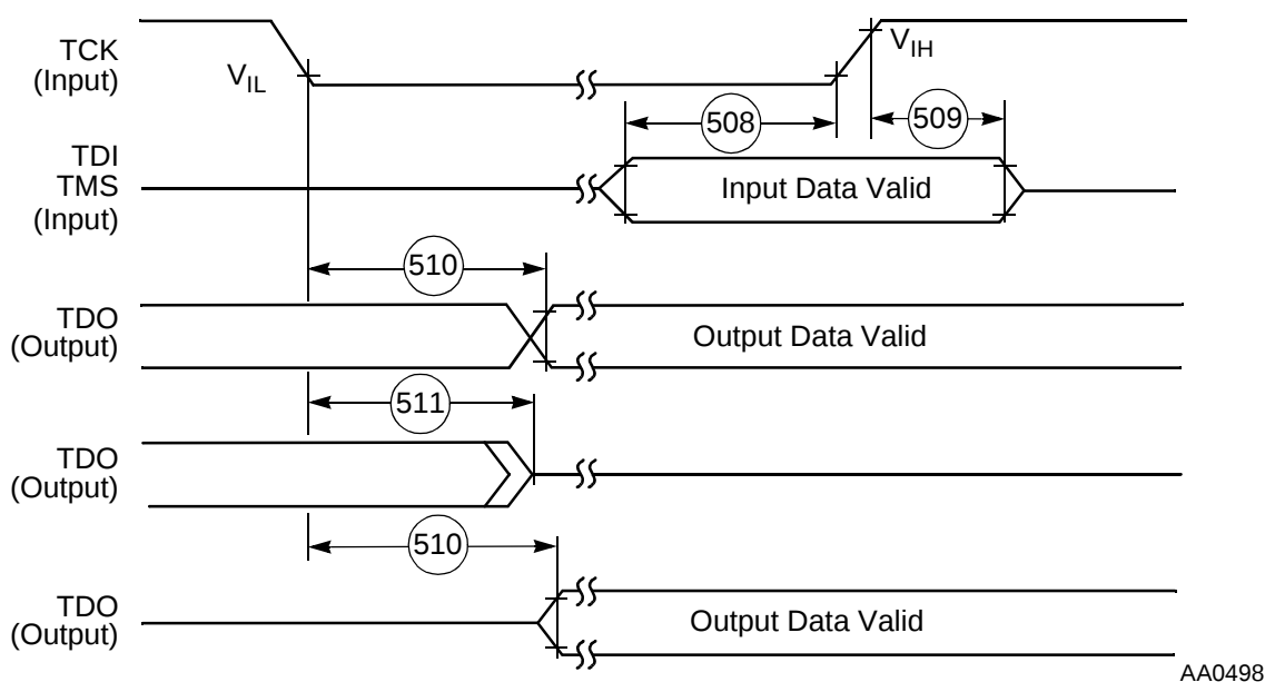
Figure 2-30. Test Access Port Timing Diagram
