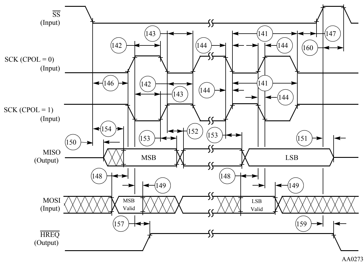
Figure 2-29 SPI Slave Timing (CPHA = 0)
