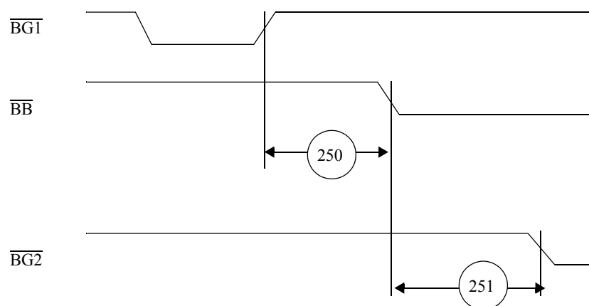
Figure 2-18 Asynchronous Bus Arbitration Timing
