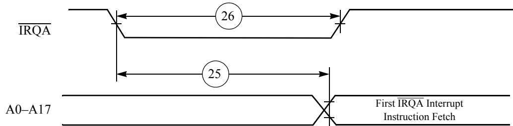
Figure 2-6 Recovery from Stop State Using \overline{IRQA}
