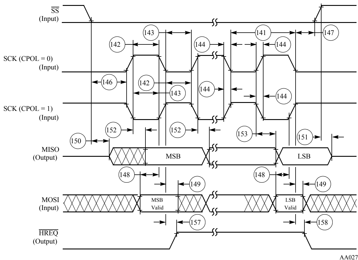
Figure 2-30 SPI Slave Timing (CPHA = 1)
