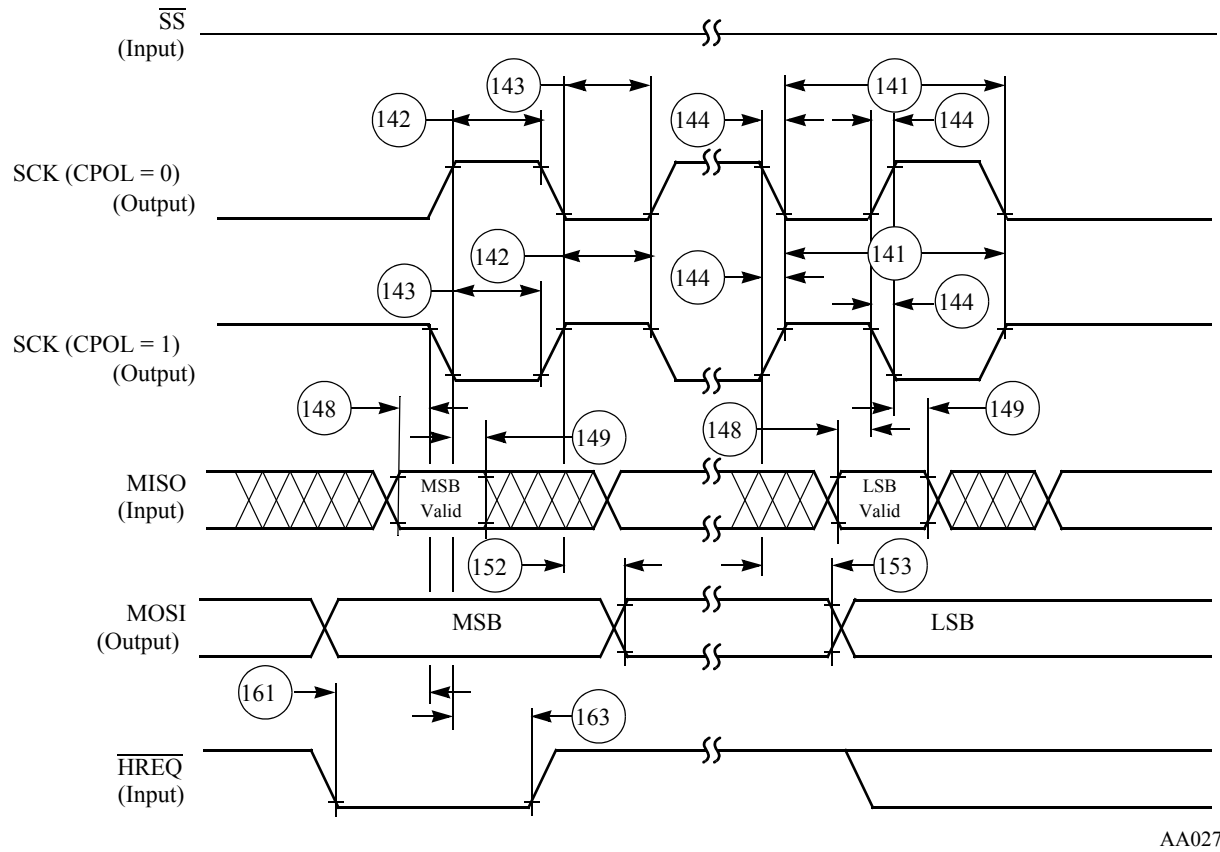
Figure 2-27 SPI Master Timing (CPHA = 0)
