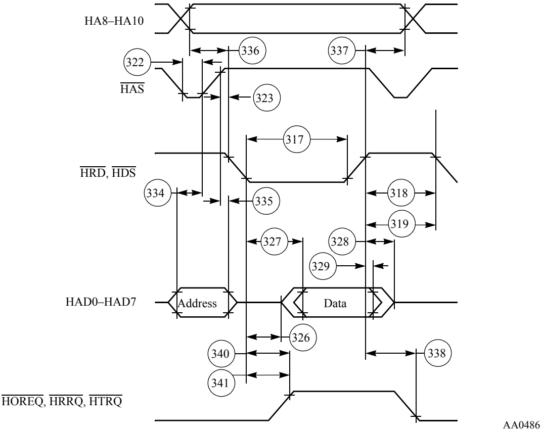
Figure 2-23 Read Timing Diagram, Multiplexed Bus
