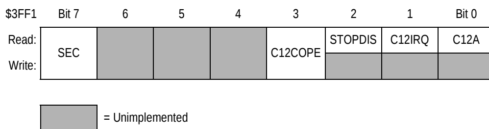
Figure 1-3. Mask Option Register 2
