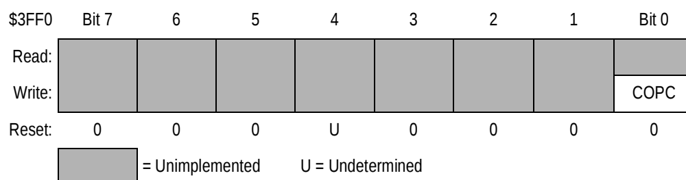
Figure 5-6. COP Clear Register (COPCLR)
