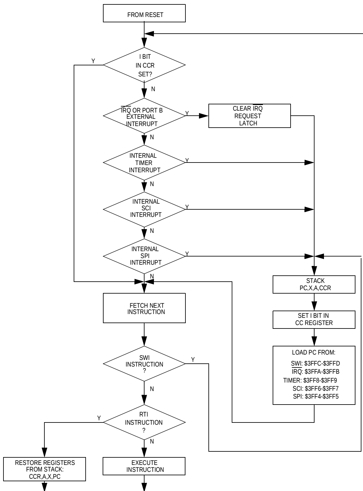
Figure 4-1. Interrupt Flowchart
