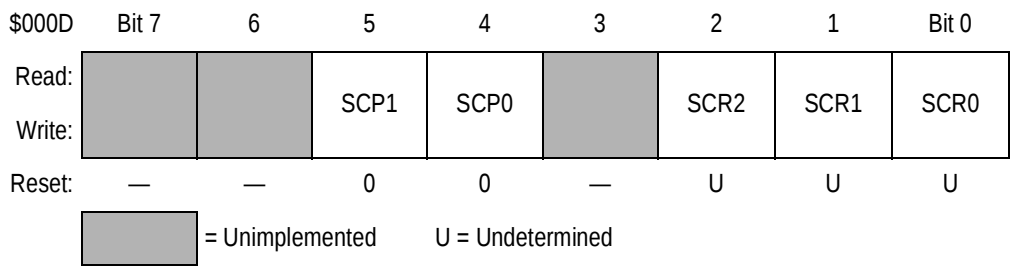
Figure 9-12. Baud Rate Register (BAUD)
